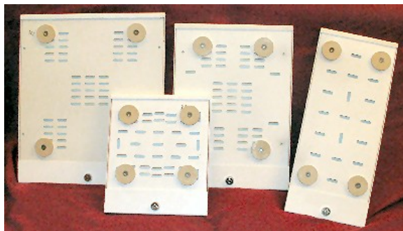
LockDown Security Plates come in standard sizes. There are two pieces: the top plate attaches to the PC using the LockDownIT adapters seen here [round pieces] and the bottom plate fixes to the furniture. The top plate with the PC slides into the bottom plate and is locked into place.
